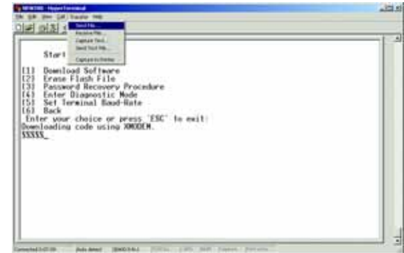
Figure C-2: Send File
