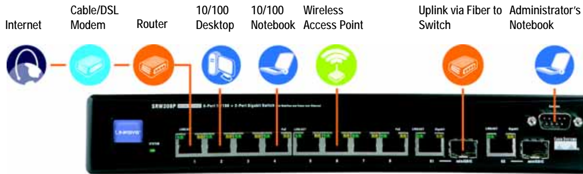
Figure 3-1: Typical Network Configuration for the SRW208P
